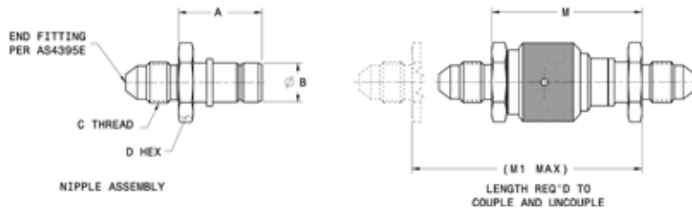
STAINLESS STEEL &amp; TITANIUM - FOR TITANIUM ADD T AS A PREFIX TO NIPPLE ASSEMBLY P/N EG: T5102-02A
